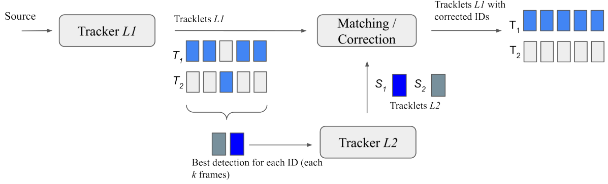
Figure 3: WindowTracker (proposal) approach overview.
