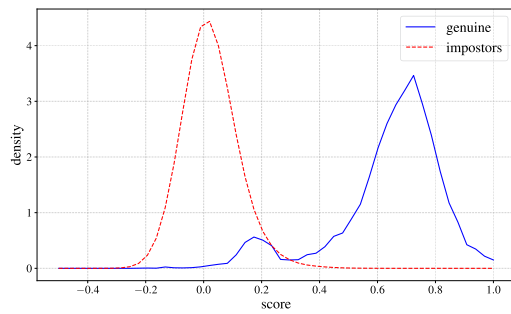
(a) Adience
