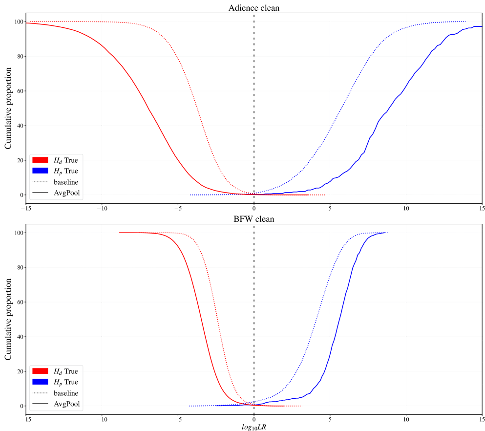
Fig. 10. Tippet plots for the Adience clean and BFW clean datasets. To avoid cluttering the figure, we only show Tippet plots for the baseline and AvgPool strategies. Tippet plots for all strategies are available in the supplementary material .
