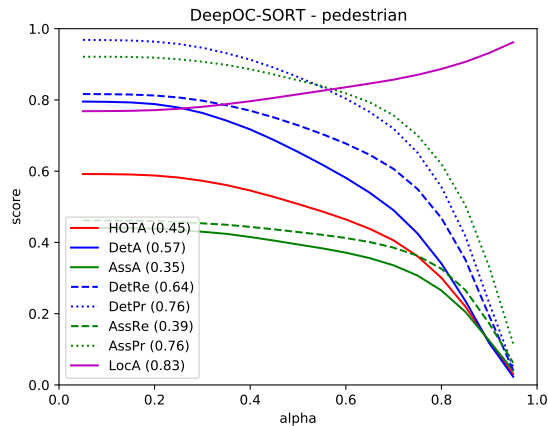
Fig. 7. HOTA Results for Deep OC-SORT
