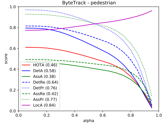
Fig. 3. HOTA Results for ByteTrack
