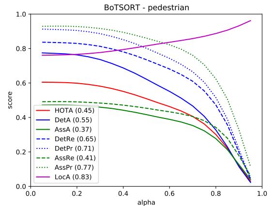
Fig. 4. HOTA Results for BotSORT
