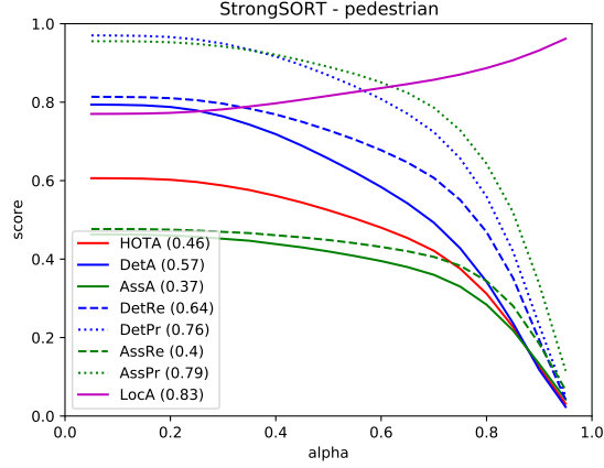
Fig. 5. HOTA Results for StrongSORT
