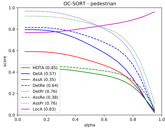
Fig. 6. HOTA Results for OC-SORT
