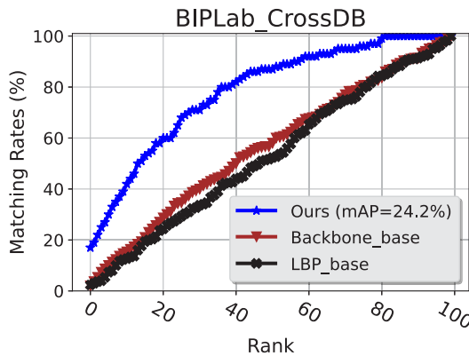
(b) CMC analysis of BIPLab with baseline methods.
