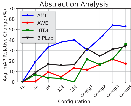
Fig. 8. Relative backbones-average mAP changes across different configurations compared to the first configuration using 16 strokes. Config1, Config2, Config3, and Config4 correspond to 16U32U64, 16U64U256, 64U128U256, and 16U32U64U128U256, respectively.
