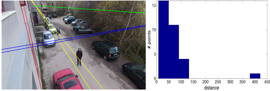
Fig. 3. Validation of the complete dual surveillance system calibration. The image on the left shows a panoramic view together with the lines defining the vanishing line (green line) and vanishing point (red lines intersection) as well as the reference height given by the distance between the two points in magenta color. On the right, the histogram shows the performance of the proposed method, when the distance d(\mathbf{r}, \mathbf{X}_1) is calculated with respect to the points selected on the heads of the people in the scene.
