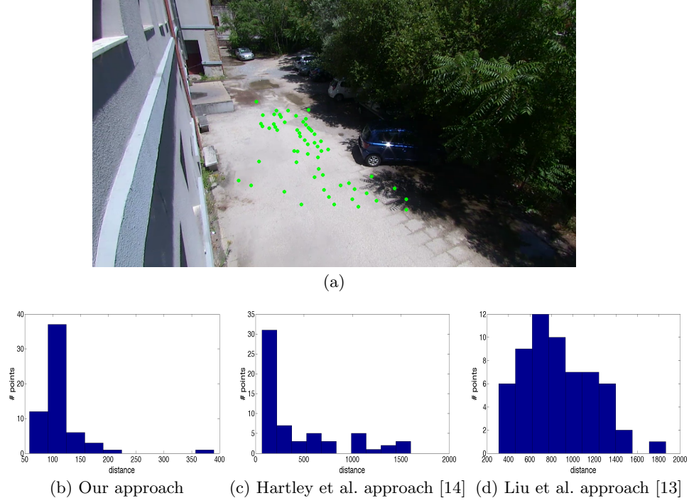
Fig. 2. Validation of the proposed dual surveillance system calibration. (a) Panoramic view given by the wide angle camera. (b), (c) and (d) show the histograms validating our approach and the models [14] and [13]. In particular, they display the number of points ( y axis) lying at several distances (in mm , x axis), according to the manually selected points ( green dots in (a)).
