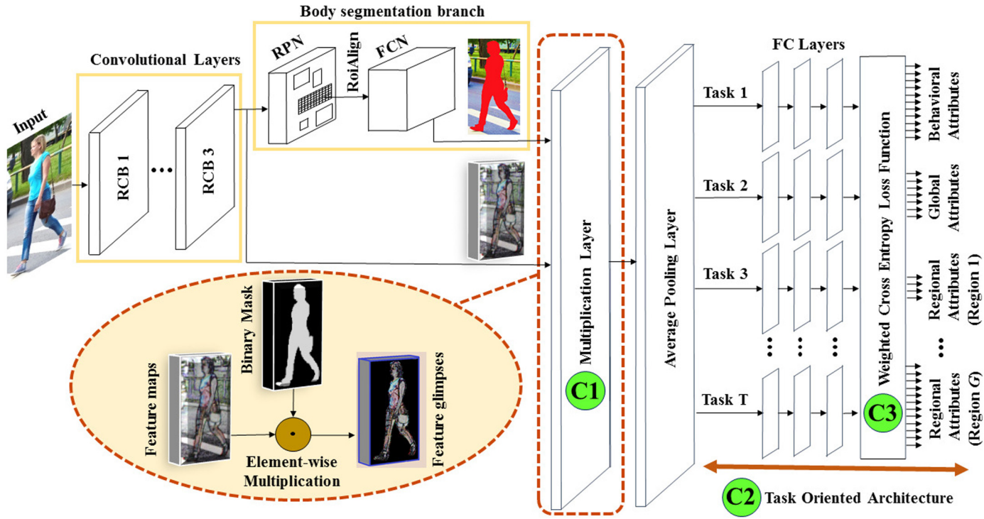
Fig. 3. Overview of the major contributions (Ci) in this paper. C1) the element-wise multiplication layer receives a set of feature maps F_{H \times W \times D} and a binary mask M_{H \times W \times D} , and outputs a set of attention glimpses . C2) The multitask-oriented architecture provides to the network the ability to focus on the local (e.g., head accessories, types of shoes), behavioral (e.g., talking, pushing), and global (e.g., age, gender) features (visual results are given in Fig. 7). C3) a weighted cross-entropy loss function not only considers the interconnection between the different attributes, but also handles the contribution of each label in the inference step. RCB is the abbreviation for Residual Convolutional Block, illustrated in Fig. 4. RPN, FCN, and FCL stand for Region Proposal Network, Fully Connected Network, and Fully Connected layer, respectively.
