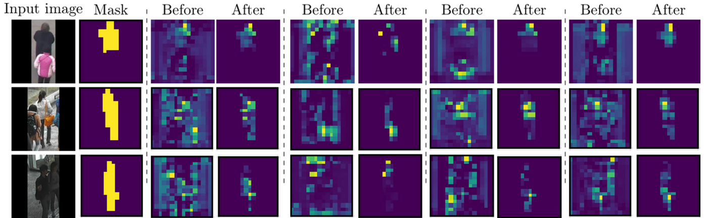
Fig. 5. The effectiveness of the multiplication layer on filtering the background features from the feature maps. The far left column shows the input images to the network, the Mask column presents the ground truth binary mask (the first input of the multiplication layer), the columns with Before label (the second input of the multiplication layer) display the feature maps before applying the multiplication operation, and the columns with After label show the output of the multiplication layer.
