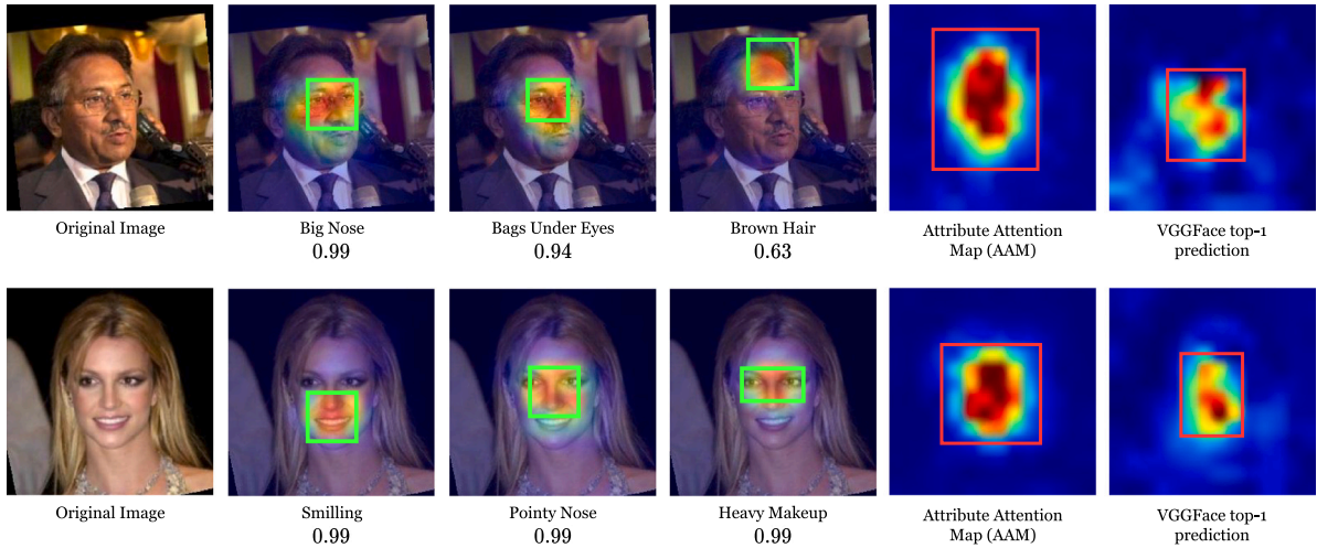
Fig. 8. Visualization of the generated Grad-CAMs for the top-3 predicted attributes of two celebrities of the LFWA dataset along with the final AAM and the heat map regarding the top-1 prediction of the VGGFace. The generated AAM contains more useful parts (wider area) concerning the face region than the reduced region illustrated in the heat map of the VGGFace top-1 prediction.
