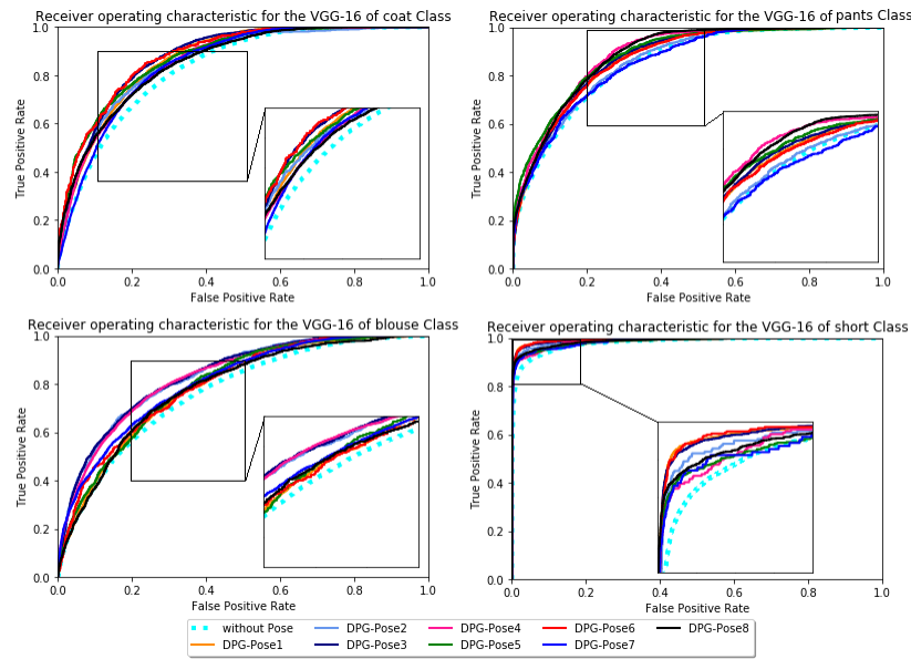
Fig. 2. ROC curves of the VGG-16 for different categories on BIODI upper-body and lower-body.
